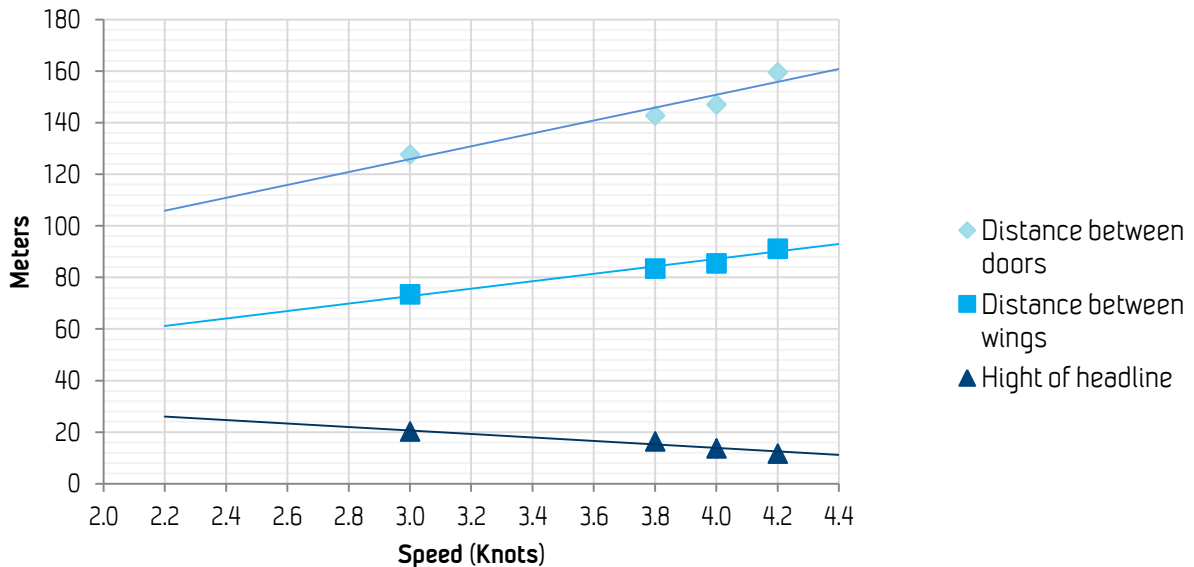
Fig 14. Geometry measurements of Y-design trawl used as semi-pelagic trawl. The trawl was rigged with 0m setback, and weight clumps of 1070kg. Warp length was approximately 840m through out the duration of the test.
