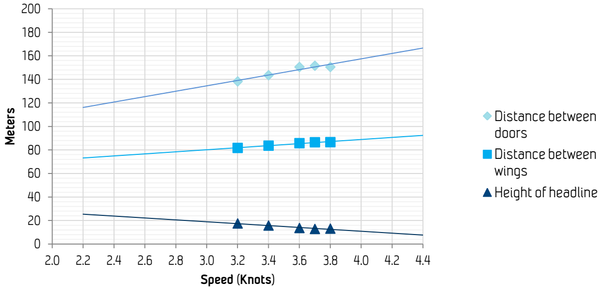
Fig 13. Geometry measurements of Y-design trawl used as semi-pelagic trawl. The trawl was rigged with 1.75m setback, and weight clumps of 1070kg. Warp length was approximately 840m through out the duration of the test.
